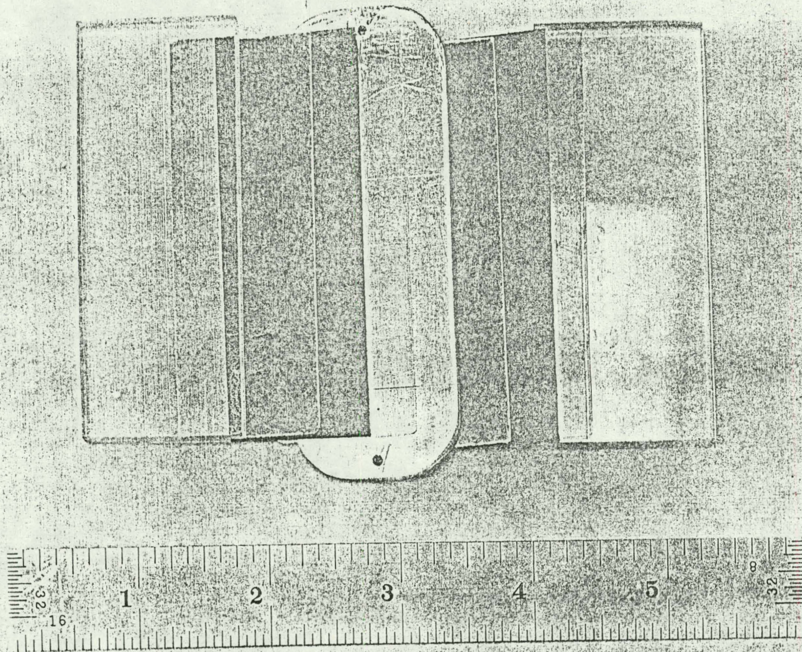
FIGURE 2. Photograph of Disassembled SSTR Neutron Dosimetry Holder. Parts are Assembled as Shown in Figure 1.
