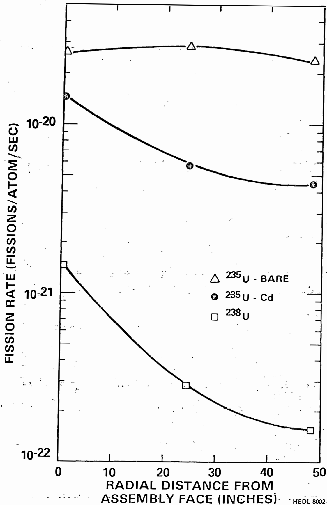
FIGURE 11. Fission Rates as a Function of Radial Distance from a Reactor (PWR) Spent Fuel Assembly.
