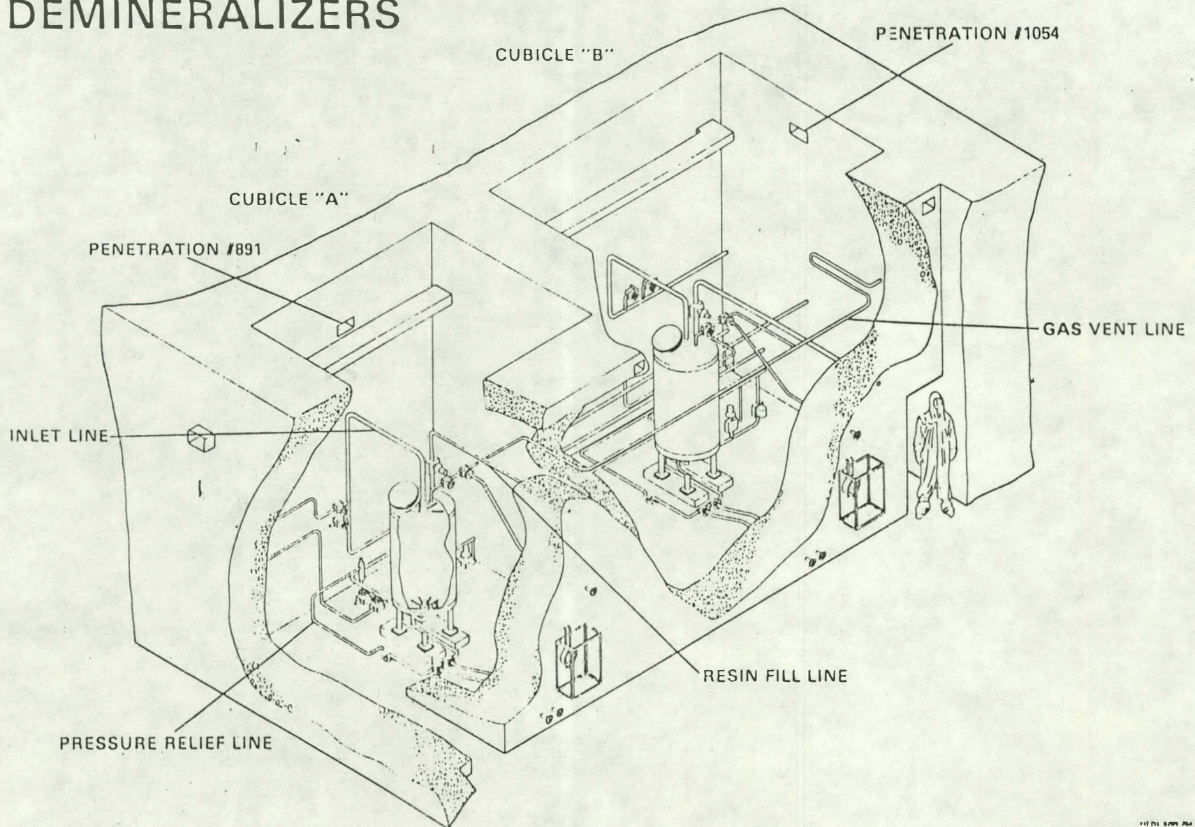
FIGURE 5. Isometric View of Makeup Demineralizer Cells A and B.
