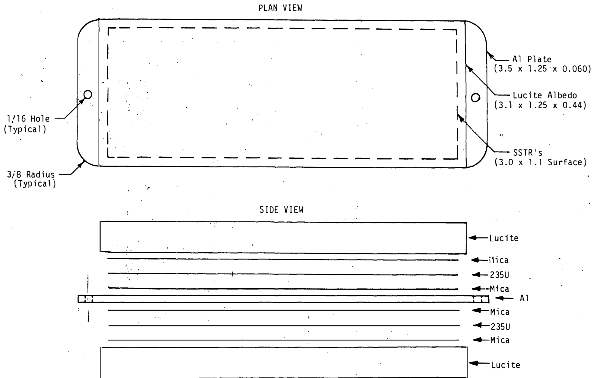
FIGURE 1. SSTR Neutron Dosimetry Holder for TMI-2 Demineralizer A Measurements.
