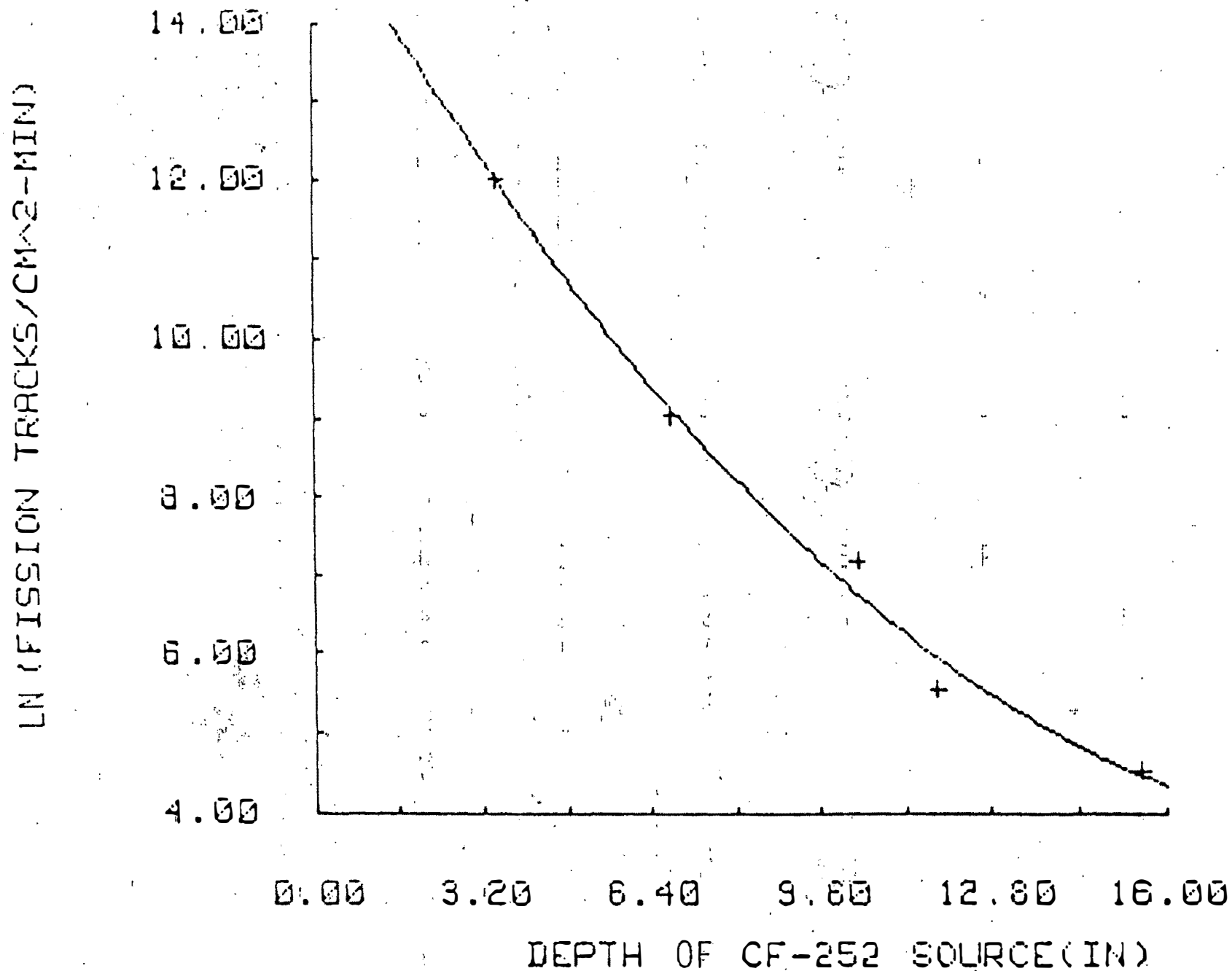
FIGURE 15. SSTR Neutron Dosimeter Response as a Function of Depth of a 252 Cf Source in 1100 ppm Borated Water.
